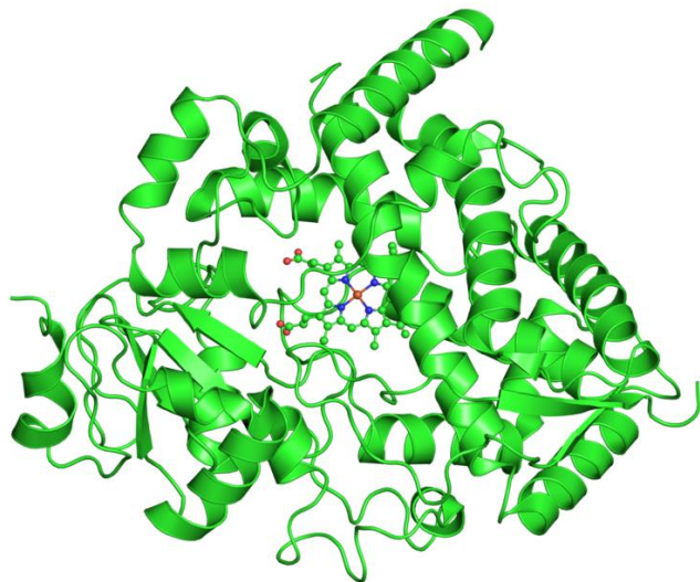
Structure of CYP3A4 Courtesy of www.ebi.ac.uk
